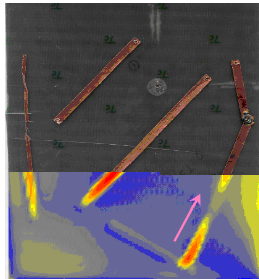
Figure 4 Test structure for resonance scanning partially overlaid with a scan result.
